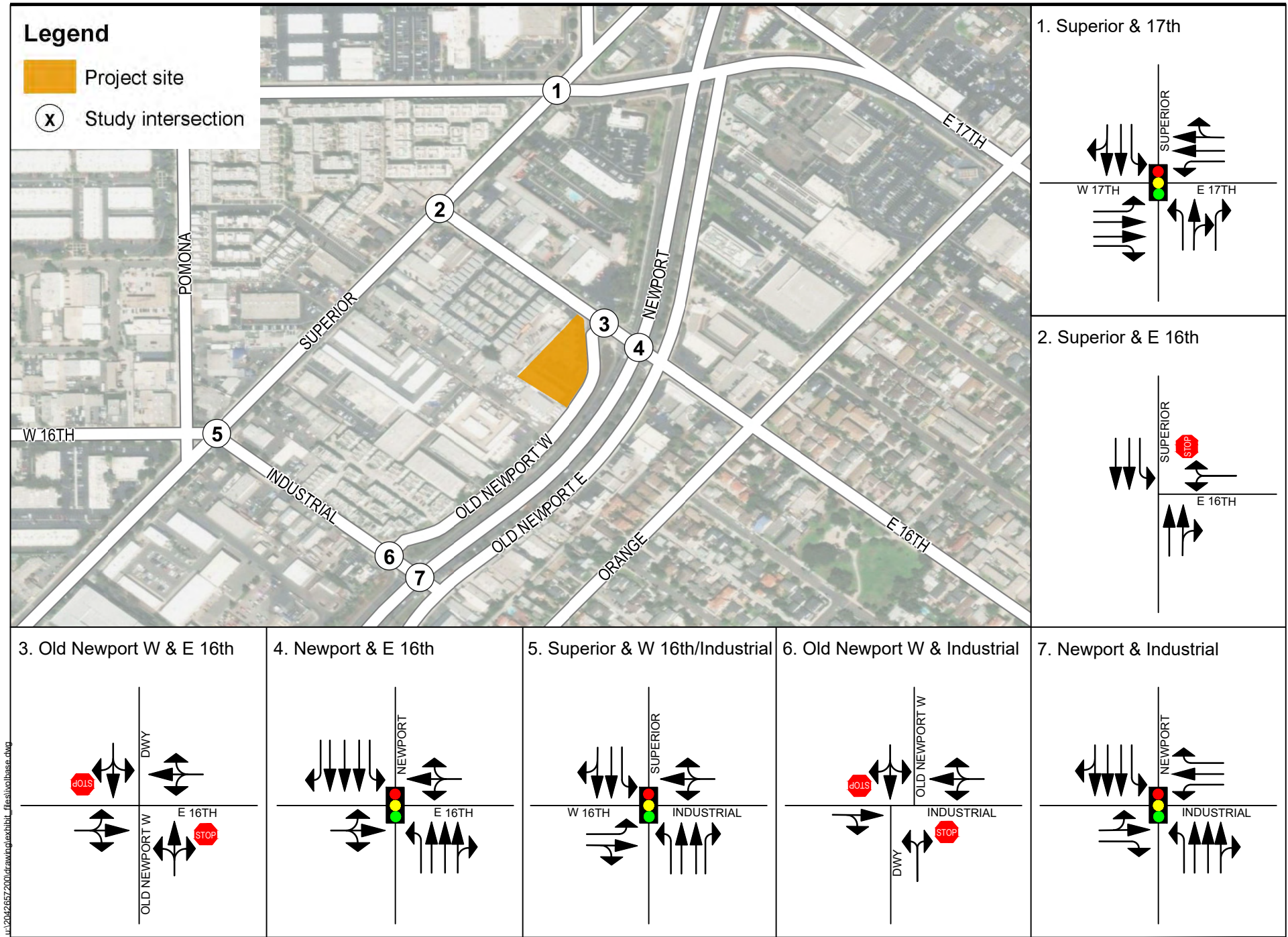
Figure 3 Existing Intersection Lane Configurations
