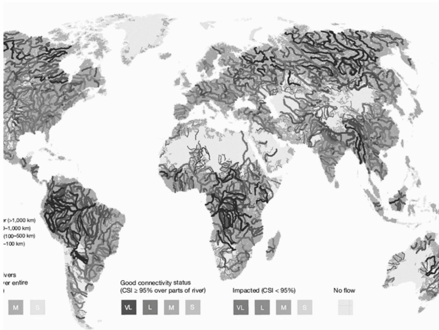
FIGURE 1 Global status of free-flowing rivers (Grill 2019).
