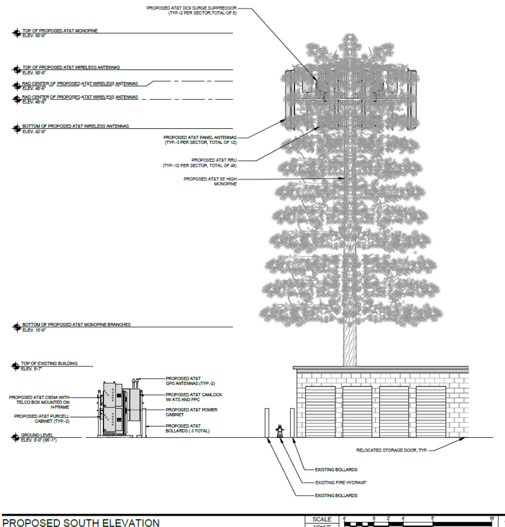
Figure 4. Elevation View
