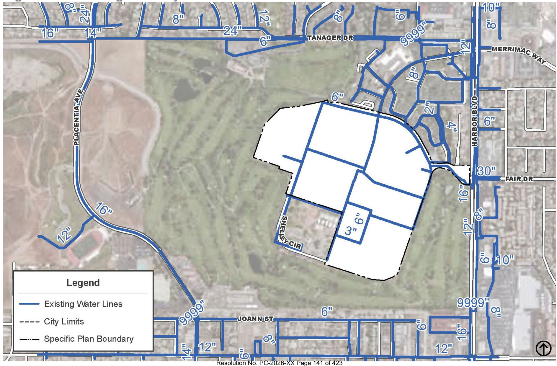
Figure 7-1: Existing Water System Facilities
