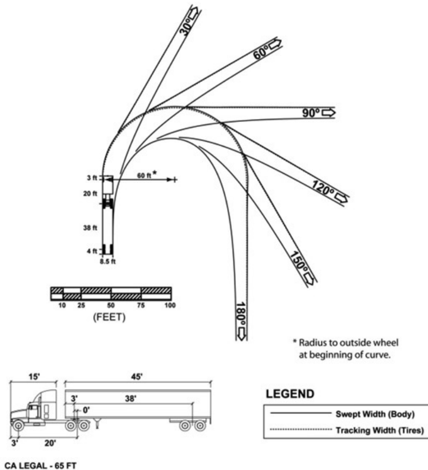
Figure 5-15: SREOC Turning Radius Vehicle Size
