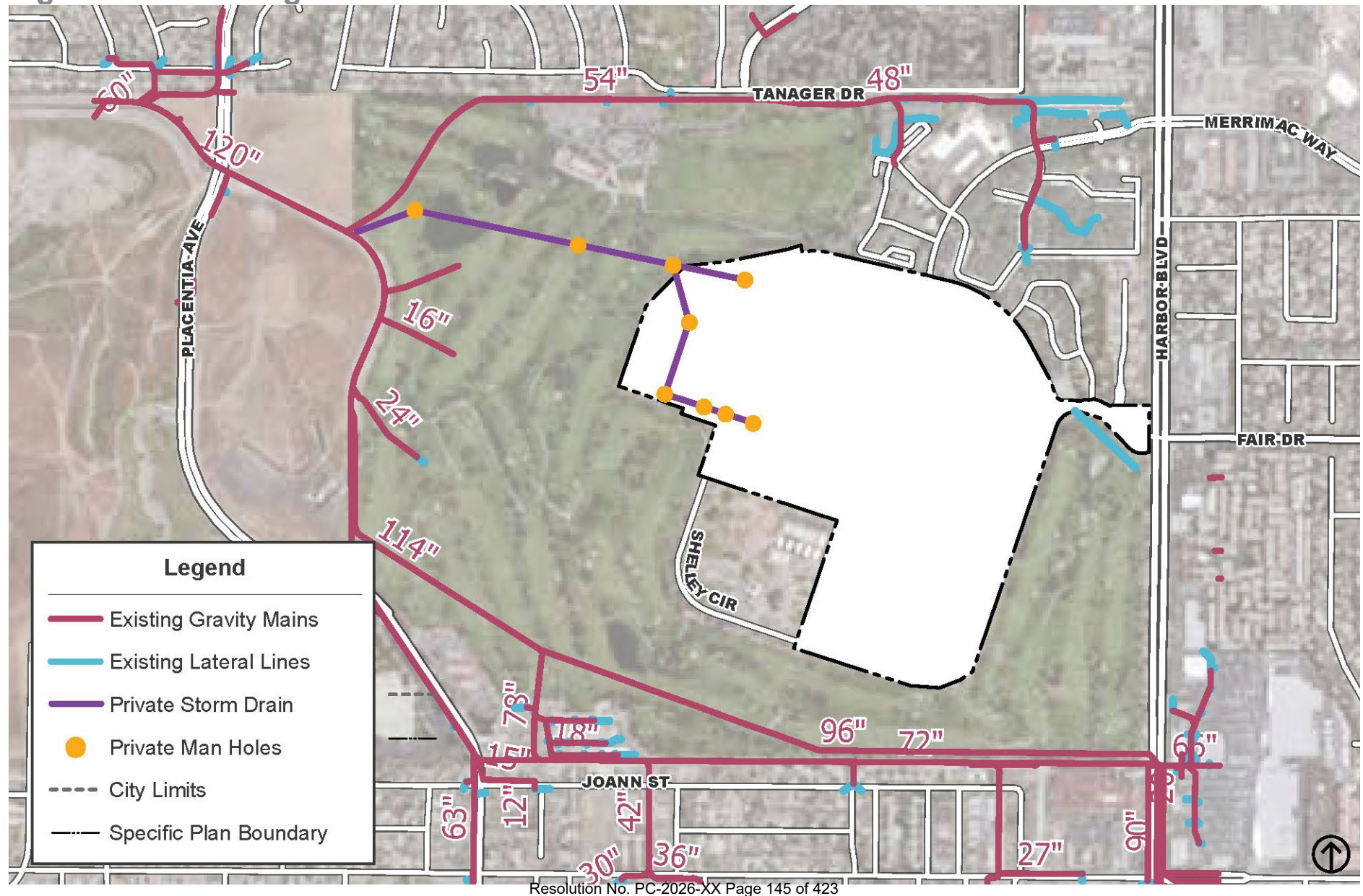
Figure 7-5: Existing Storm Drain Facilities
