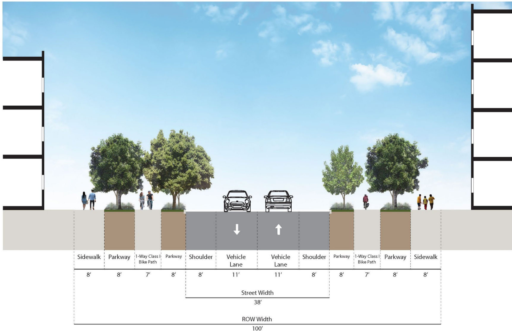
Figure 5-5: Promenade Street Section Option 2
