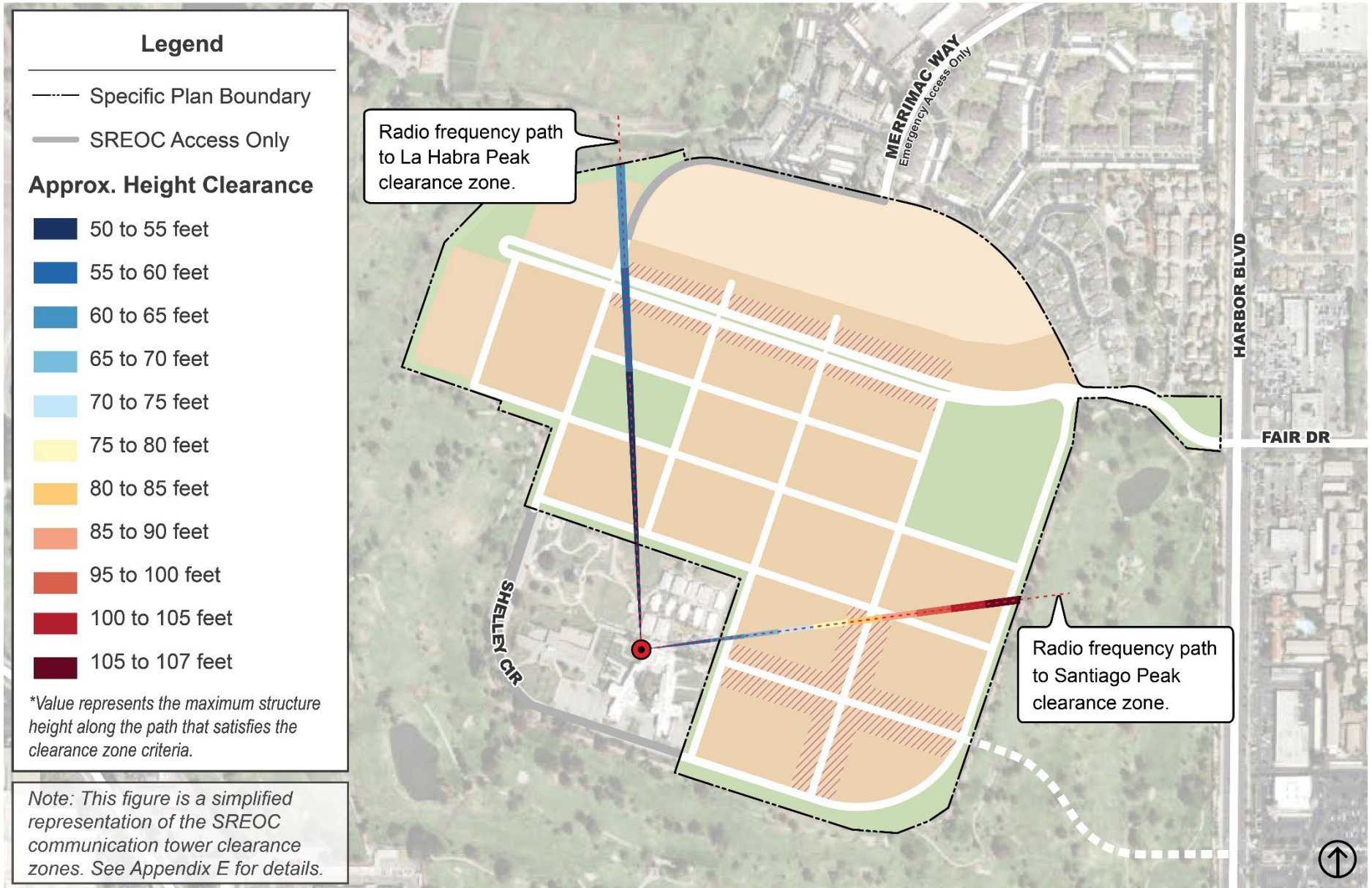
Figure 4-4: SREOC Tower Location and Antenna Clearance
