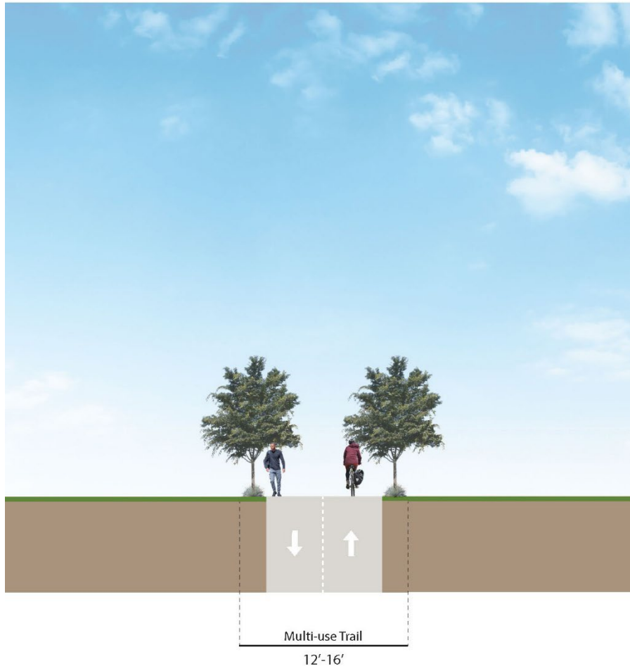
Figure 5-11: Multi-Use Trail Section
