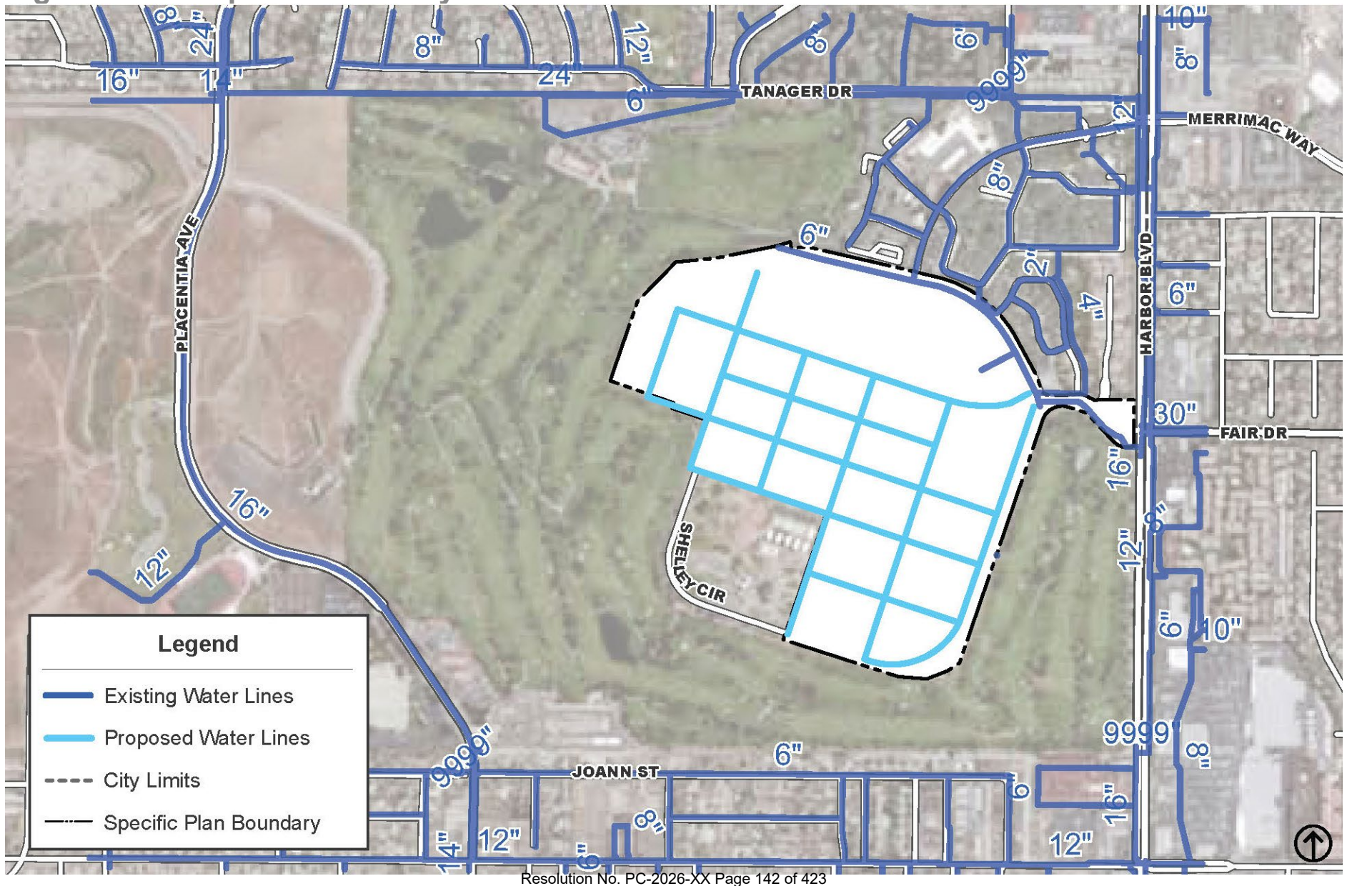
Figure 7-2: Proposed Water System Facilities
