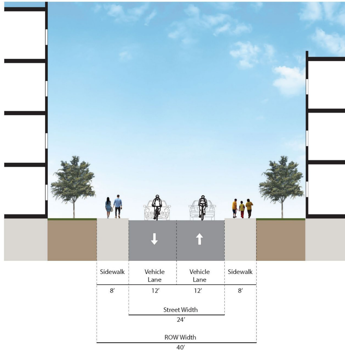
Figure 5-9: Local Road, No Parking Street Section
