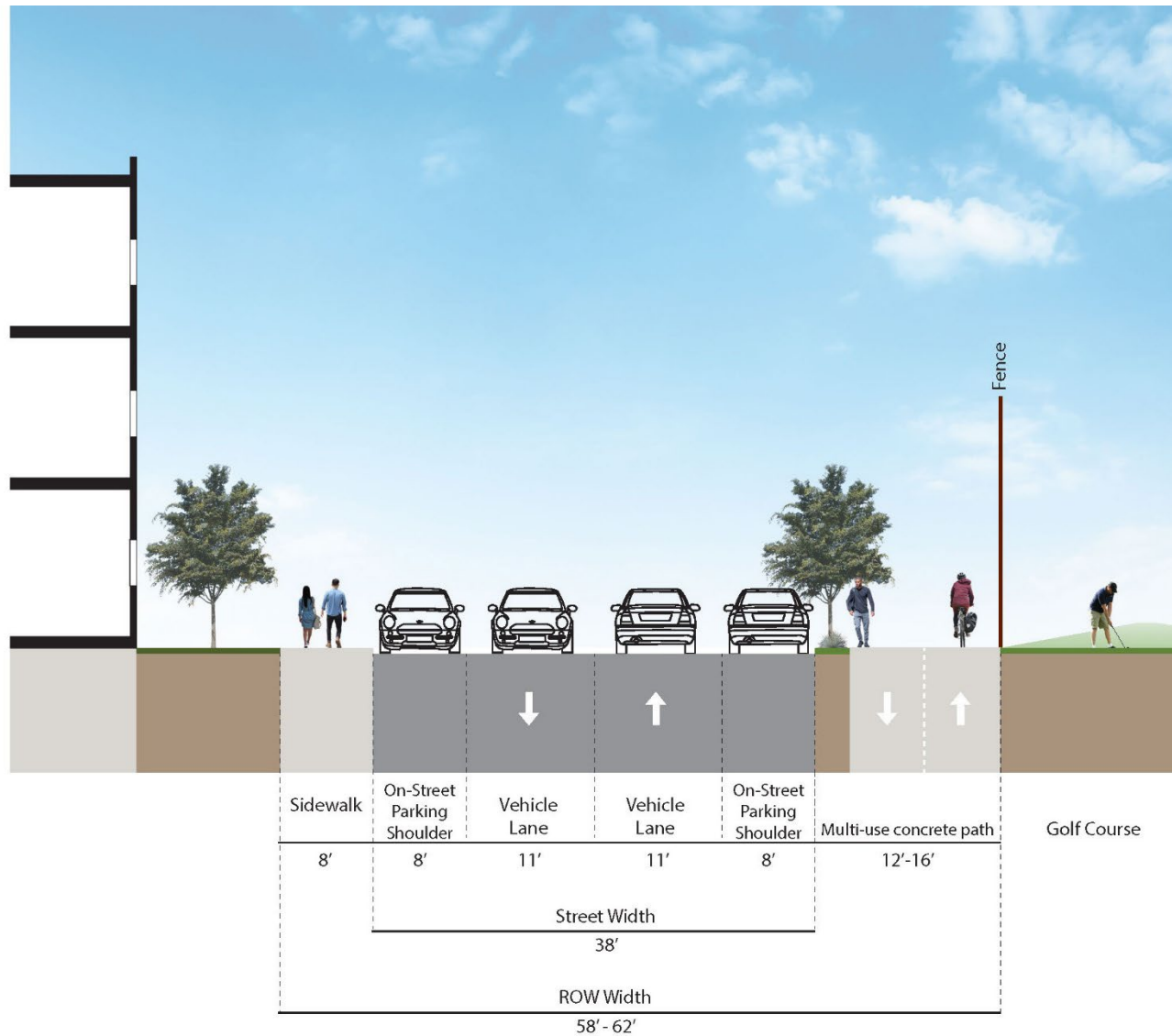
Figure 5-6: Shelley Circle Street Section
