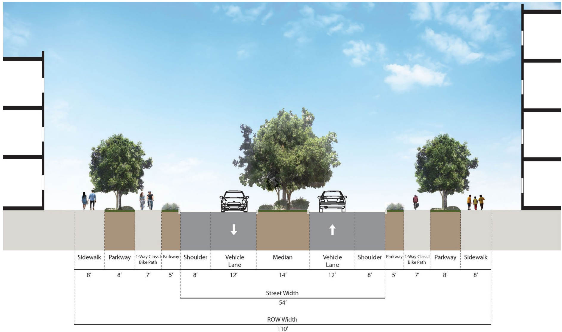
Figure 5-4: Promenade Street Section Option 1
