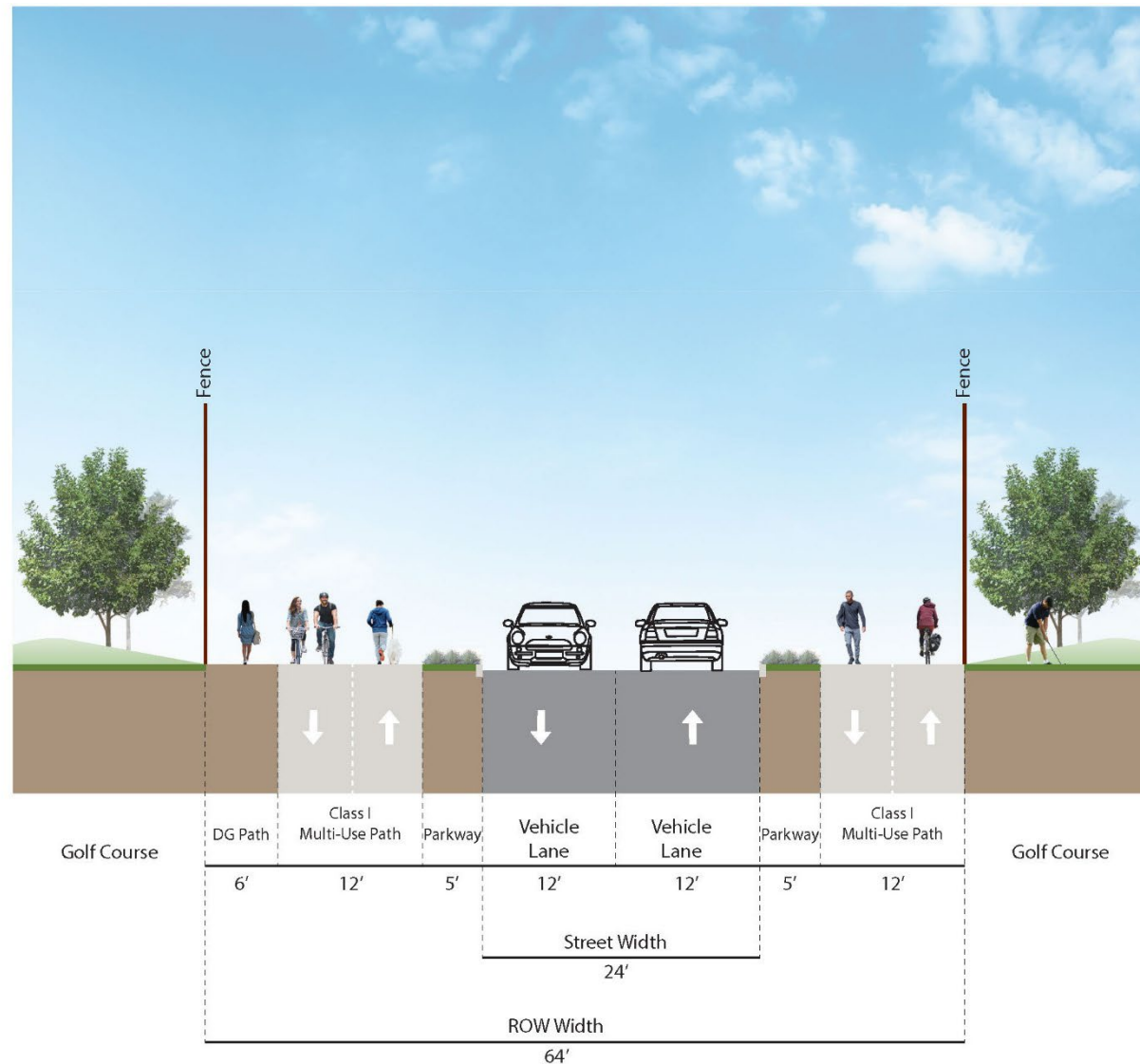
Figure 5-8: Secondary Access through the Golf Course Option 2
