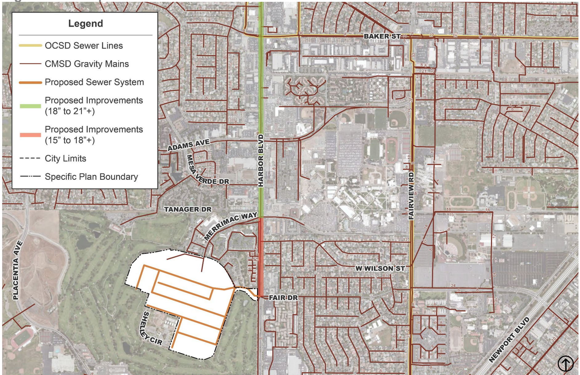
Figure 7-4: Proposed Sewer Facilities
