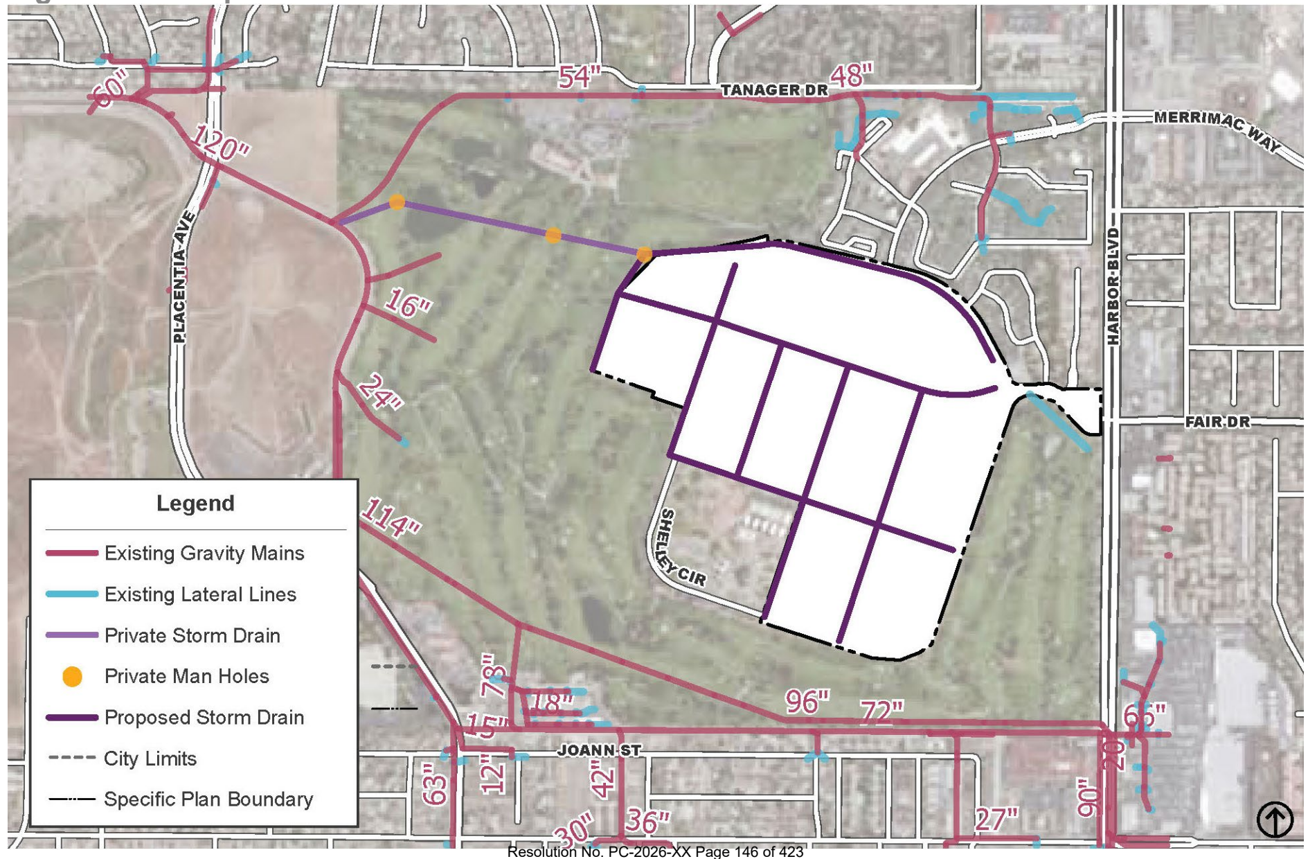
Figure 7-6: Proposed Storm Drain Facilities
