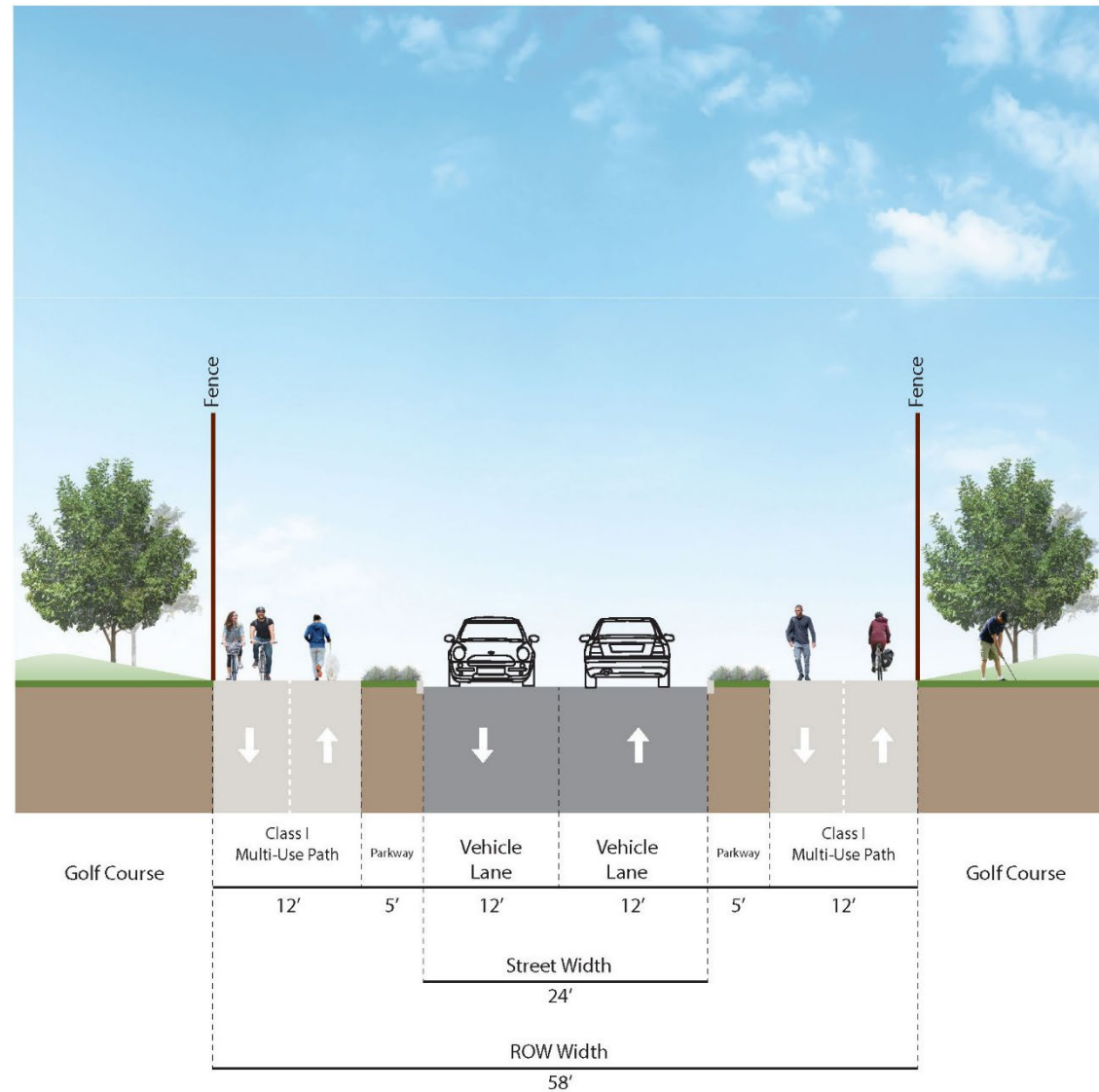
Figure 5-7: Secondary Access through the Golf Course Option 1
