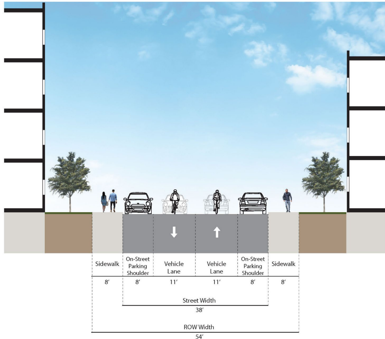
Figure 5-10: Local Road with Parking Street Section
