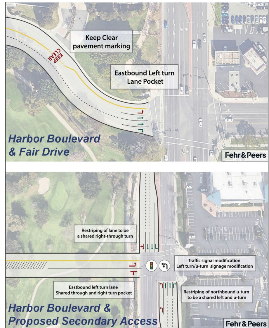
Figure 5-14: Intersection Improvements
