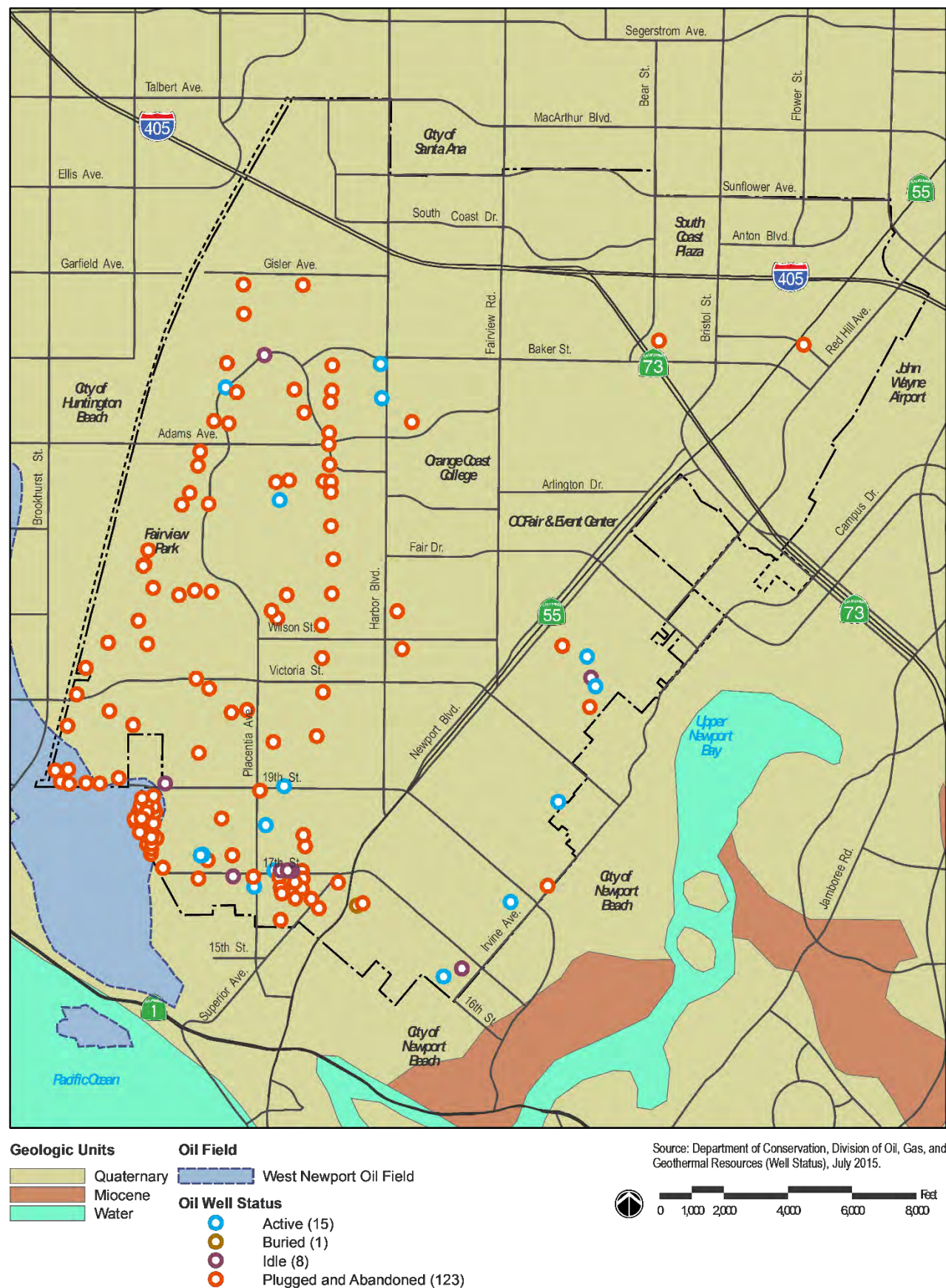
Figure S-1: Geologic Units
